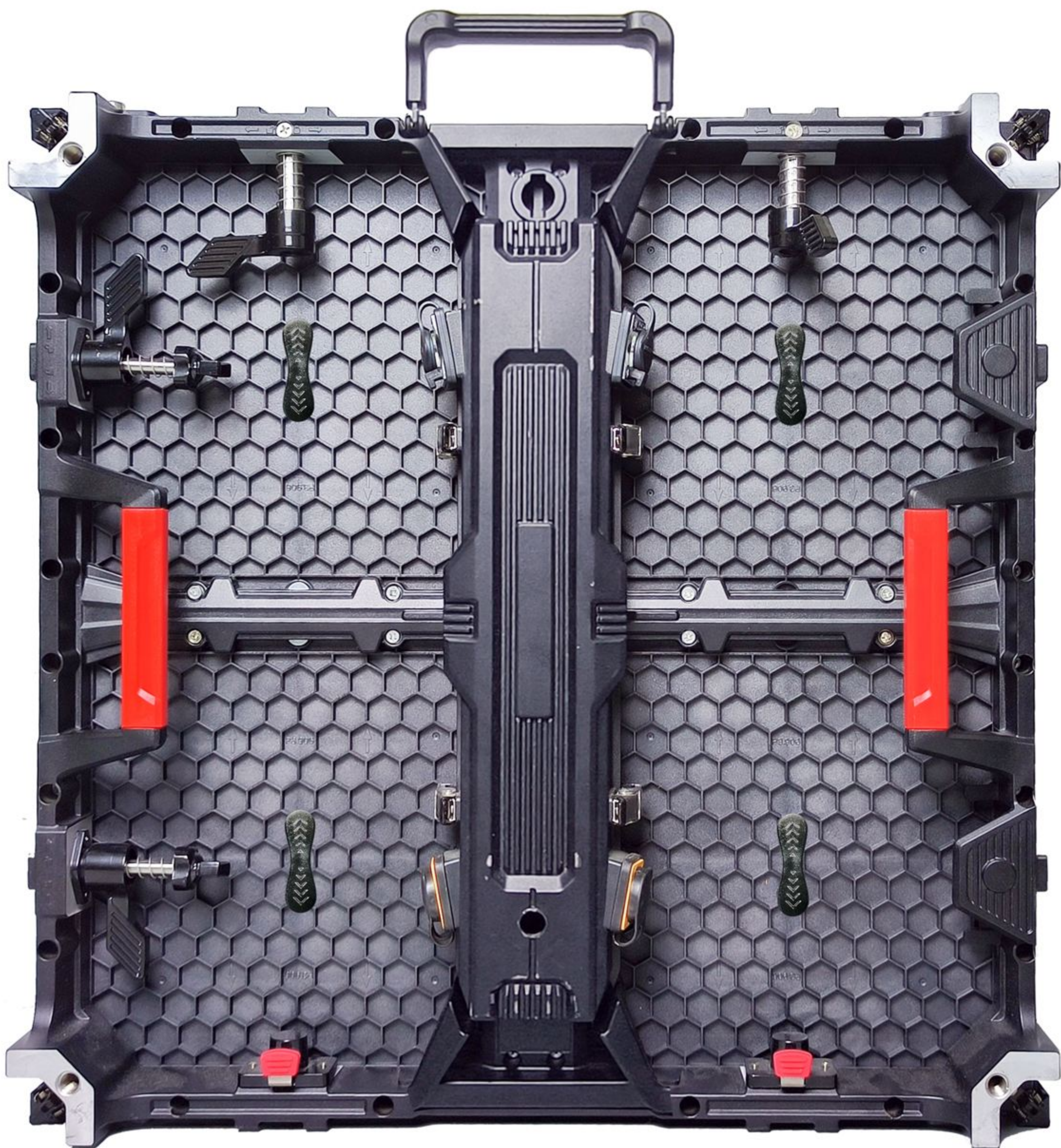
Back View
